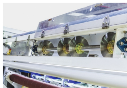
Edge tape cutting structure 边条分切结构
