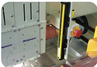
Safety Light Curtain
