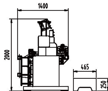
Automatic Receiving Rack
