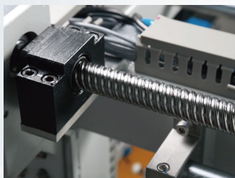
Lead screw drive
