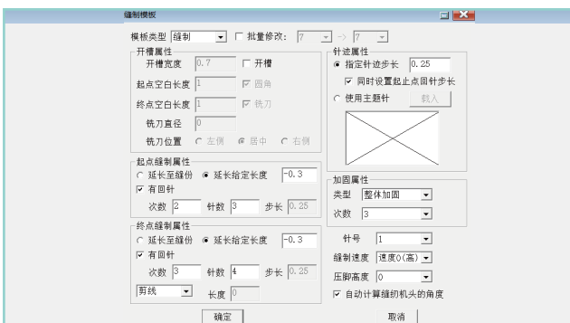
单界面设计针迹线，包括倒针、回针、锁针、针步长短等 Single-interface stitching design, including backstitch, return stitch, lock stitch, and stitch length settings.
