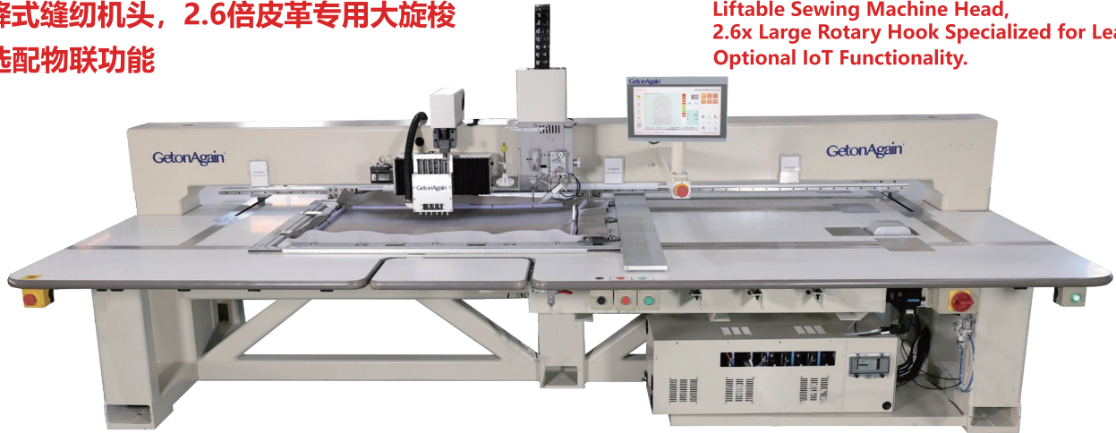
GOACE-L-P+S-1-900x600-B-P6+IS2-HR2.6-LH50,AO-1P220
