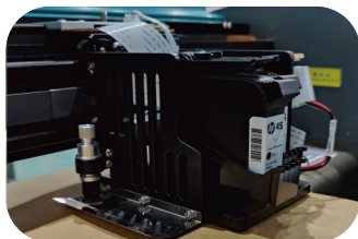
喷切机头 Inkjet cutting head
