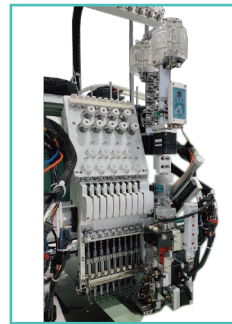
2色散珠装置 2 Colors Beading Device
