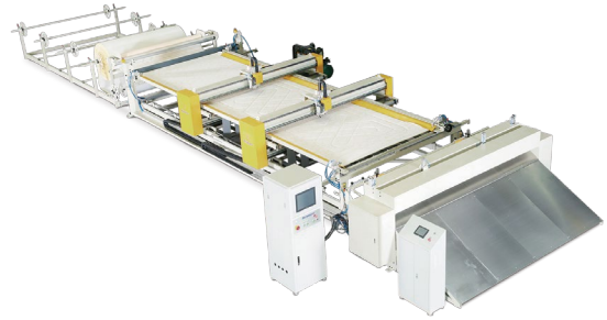
连续送料龙门式绗缝机-双鞍架(撑布带) Continuous Feeding Double Saddles Quilting Machine (with Supporting Belt)
