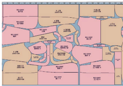
混合排料 Mixing Nest
