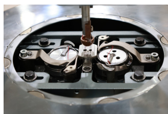
3倍超大旋梭 3X Oversized Rotary Hook
