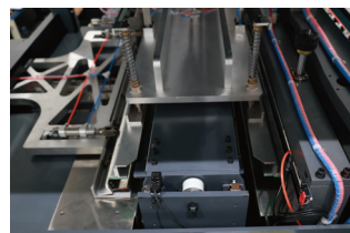
压料装置 Pressing Device Ensure Towels
