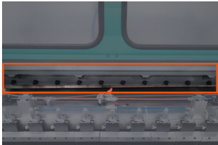
定长裁切机构 Preset Length Cutting Mechanism
