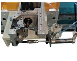
稳定可靠的动刀剪线系统 Stable and reliable moving knife for thread trimming system
